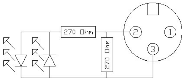
3-PIN DMX TESTER & TERMINATOR
