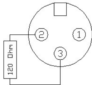
3-PIN DMX TESTER & TERMINATOR
