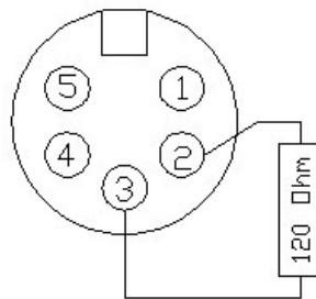
5-PIN DMX TESTER & TERMINATOR
