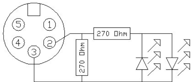
5-PIN DMX TESTER & TERMINATOR
